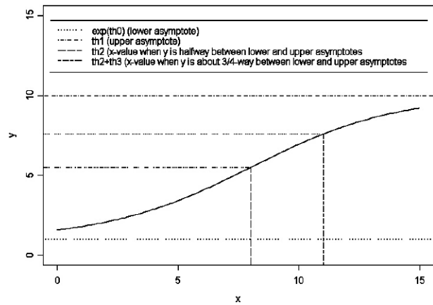
FIG. 1. An example of the four parameter logistic curve with components \theta_0 , \theta_1 , \theta_2 , and \theta_3 (0, 10, 8 and 3, respectively).
